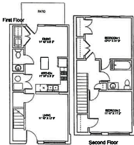
2 BR/1.5Bath Townhouse
